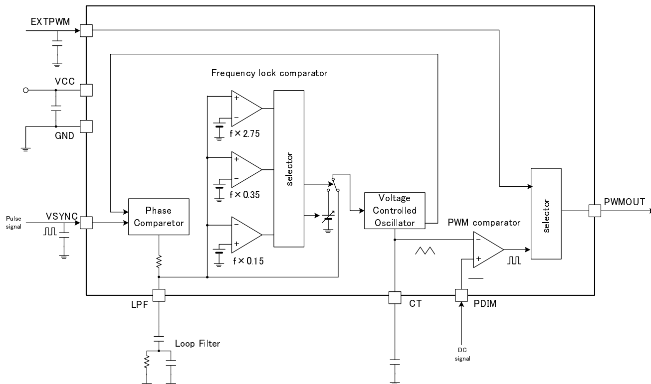
Figure 6. Block Diagram
