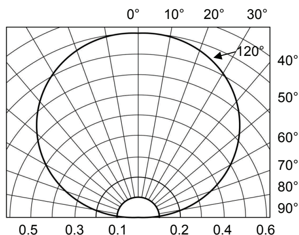
Fig. 2 Directivity Radiation Diagram
