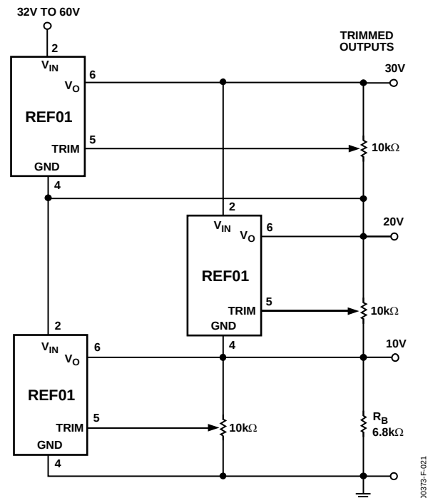
Figure 21. Reference Stack
