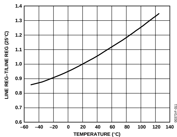
Figure 9. Normalized Line Regulation vs. Temperature
