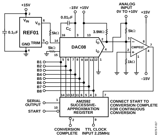
Figure 17. DAC Reference
