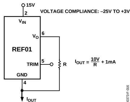
Figure 16. Current Source
