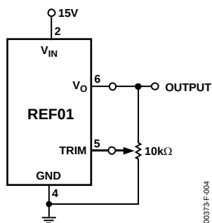
Figure 12. Output Adjustment
