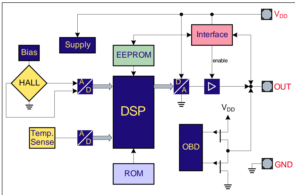
Figure 2 Block Diagram
