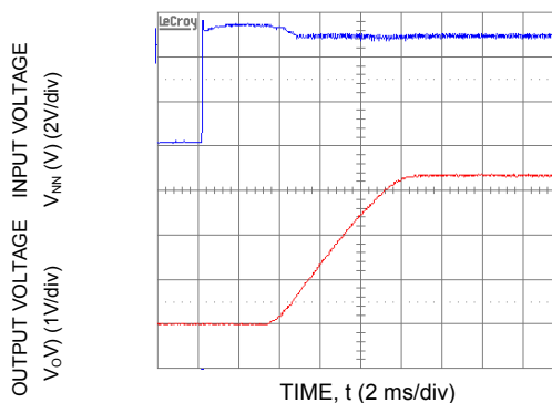
Figure 16. Typical Start-Up with application of V_{in} ( V_{in} = 5.5\text{ Vdc} , V_o = 3.3\text{ Vdc} , I_o = 10\text{ A} ).
