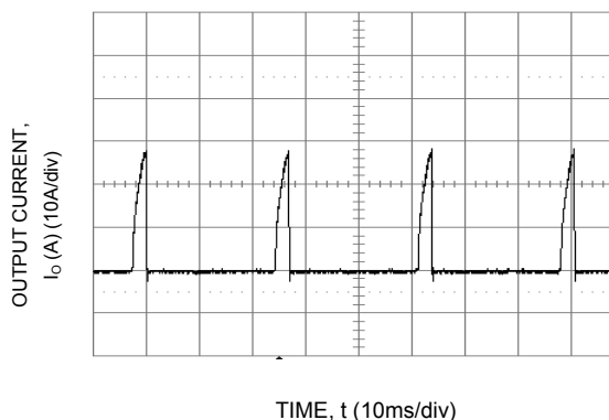
Figure 18. Output short circuit Current ( V_{in} = 5.0\text{ Vdc} , V_o = 0.75\text{ Vdc} ).
