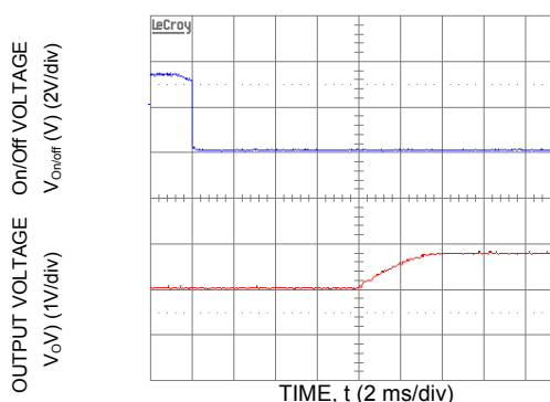
Figure 17. Typical Start-Up with Prebias ( V_{in} = 5.5\text{ Vdc} , V_o = 1.8\text{ Vdc} , I_o = 1\text{ A} , V_{bias} = 1.0\text{ Vdc} ).
