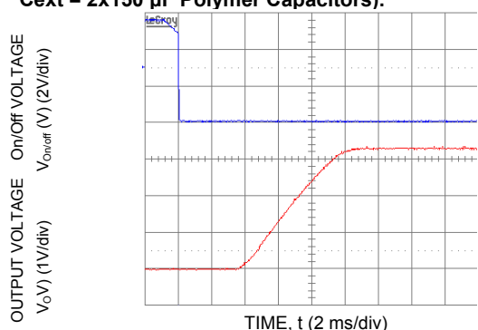
Figure 14. Typical Start-Up Using Remote On/Off ( V_{in} = 5.5\text{ Vdc} , V_o = 3.3\text{ Vdc} , I_o = 10\text{ A} ).
