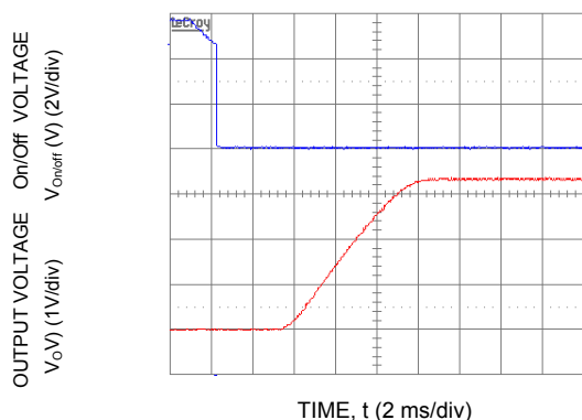
Figure 15. Typical Start-Up Using Remote On/Off with external capacitors ( V_{in} = 5.5\text{ Vdc} , V_o = 3.3\text{ Vdc} , I_o = 10\text{ A} , C_o = 1050\text{ }\mu\text{F} ).
