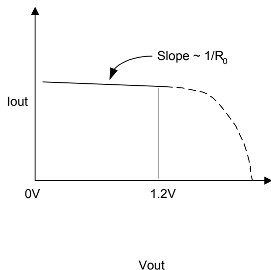
Figure 4. Buffer Characteristics
