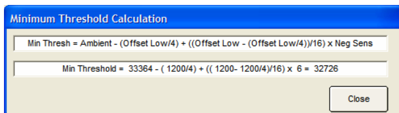
Figure 13. Minimum Threshold Formula
