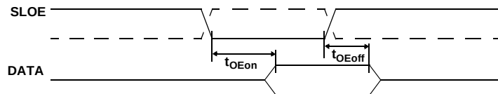
Figure 9-11. Slave FIFO Output Enable Timing Diagram [12]
