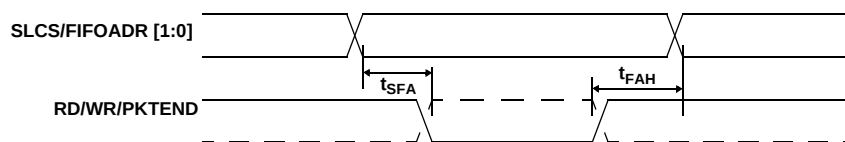
Figure 9-14. Slave FIFO Asynchronous Address Timing Diagram [12]
