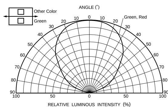
Fig. 2 Directional pattern (2)
