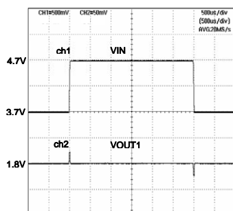
Fig.37. VIN Response (VOUT1=1.8V) IOUT=50mA
