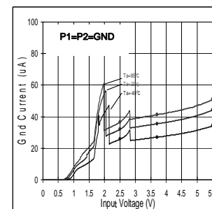
Fig.12. Circuit Current (VOUT1=1.8V, VOUT2=2.9V) EN1=GND, EN2=VIN
