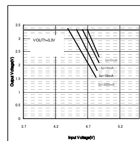
Fig.9. Line Regulation (VOUT1=3.3V)
