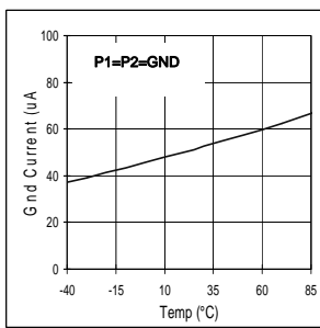
Fig.23. Icc - Temp (VOUT1=1.8V, VOUT2=2.9V) EN1=EN2=VIN
