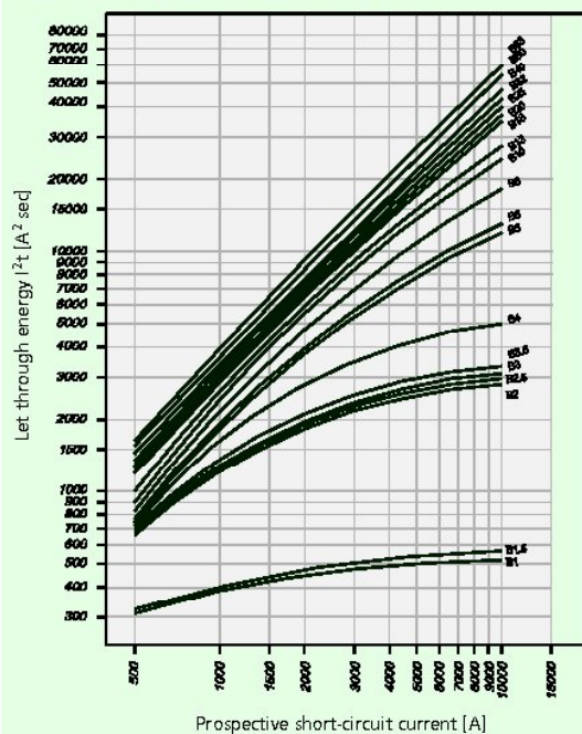
Let-through energy PLSM, characteristic B, 1-pole
