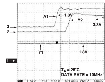
TPC 27. Bypass Mode, V_{CC1} = 1.8\text{ V} , V_{CC2} = 3.3\text{ V}
