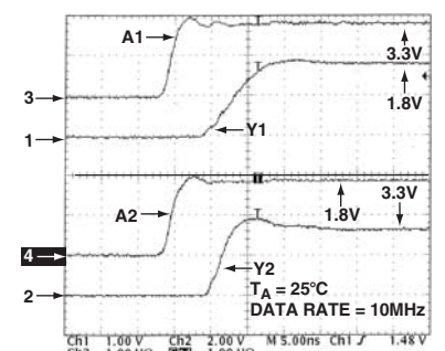
TPC 26. Normal Mode V_{CC1} = 1.8\text{ V} , V_{CC2} = 3.3\text{ V}
