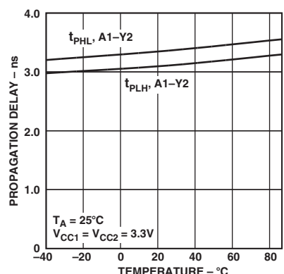
TPC 23. Propagation Delay vs. Temperature, Bypass Mode
