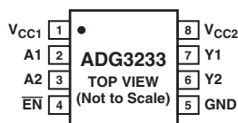
8-Lead SOT-23 Package (RJ-8)
