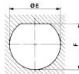
Jam nut receptacle (type 7)
