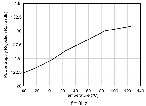
Figure 5-16. PSRR vs Temperature (dB)
