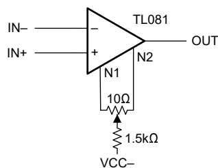
Figure 6-4. Test Figure 4 (for SO Package Only)
