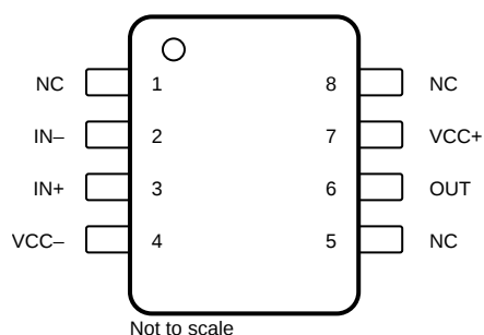
Figure 4-3. TL081x: D Package, 8-Pin SOIC, P Package, 8-Pin PDIP (Top View)
