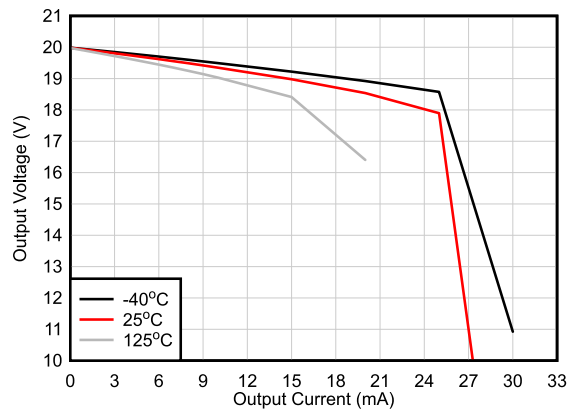
Figure 5-13. Output Voltage Swing vs Output Current (Sourcing)
