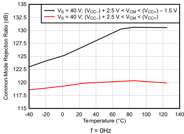
Figure 5-15. CMRR vs Temperature (dB)
