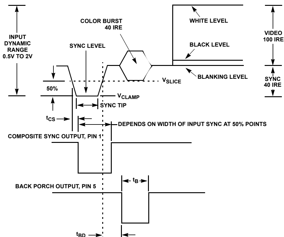
FIGURE 12. STANDARD (NTSC INPUT) H. SYNC DETAIL
