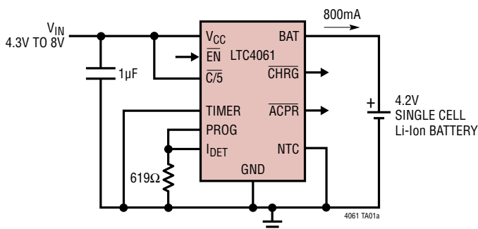
800mA Single Cell Li-Ion Battery Charger (C/10 Termination)
