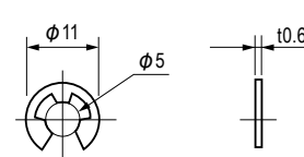
E 形止め輪 E-shaped Snap Ring
