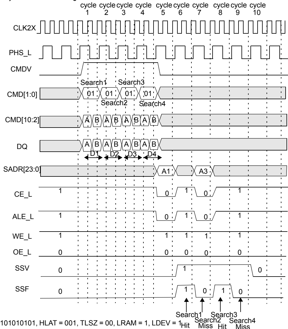
Figure 10-27. Timing Diagram for 144-bit Search (One Device)
