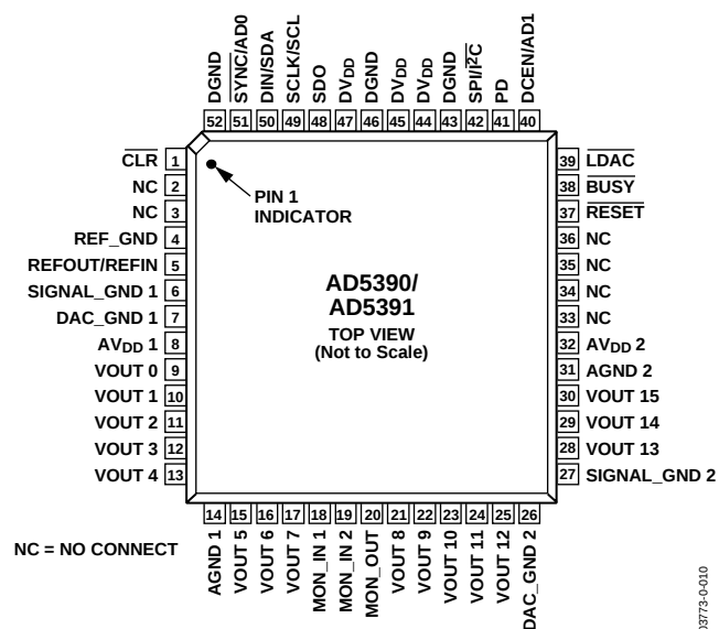
Figure 9. AD5390/AD5391 LOFP Pin Configuration
