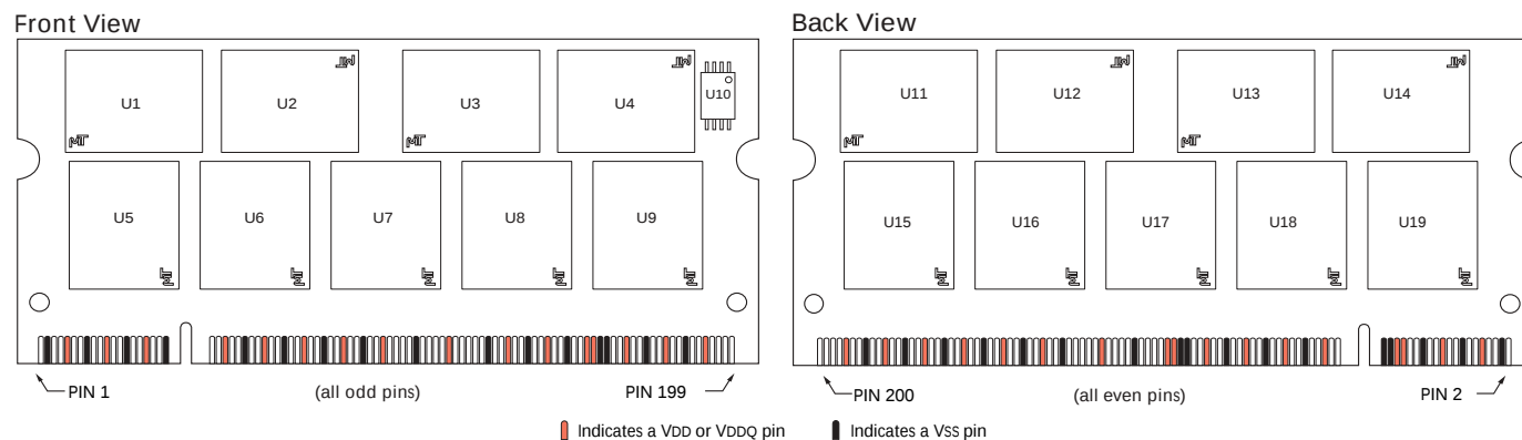
Figure 2: Module Layout
