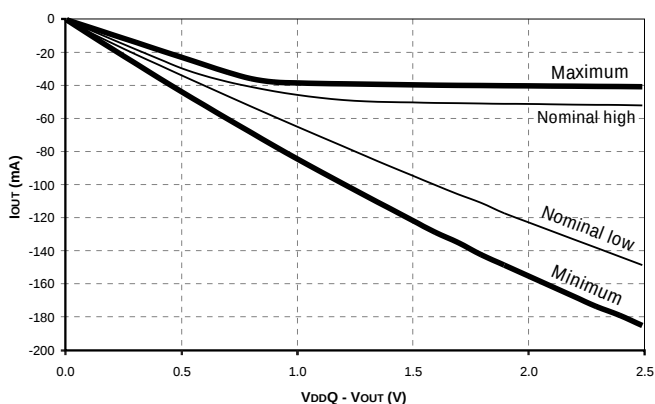
Figure 8: Pull-Up Characteristics
