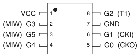
Figure 3: ACE1001 TSSOP 8-Pin Device Pinout (a) Normal Operation
