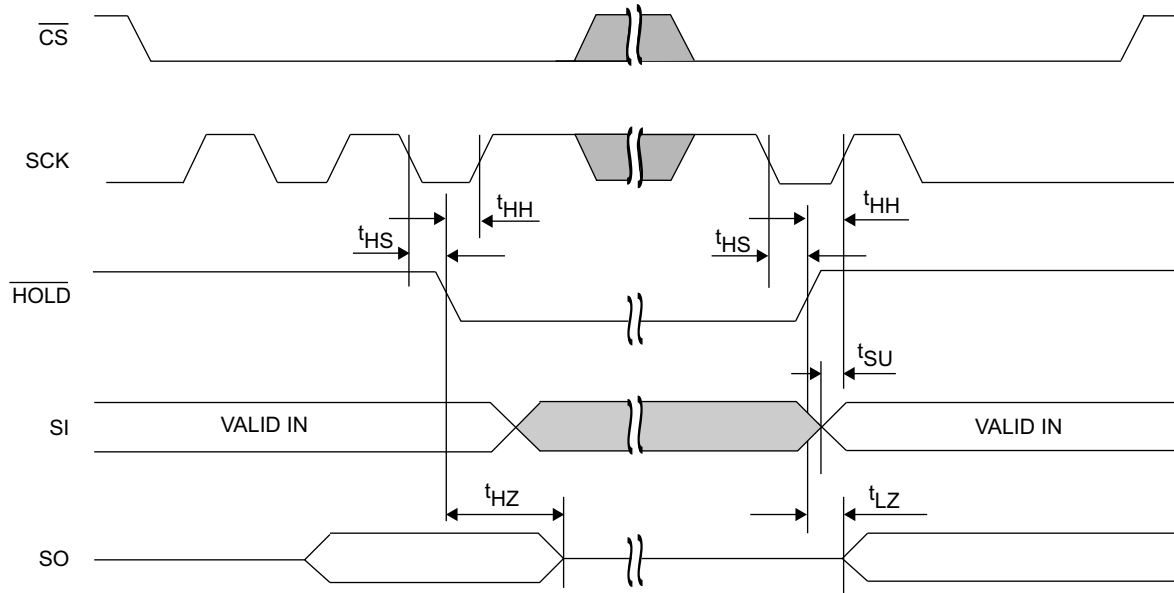
Figure 18. \overline{HOLD} Timing
