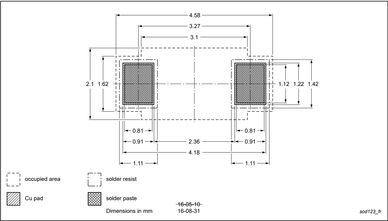
Fig. 9. Reflow soldering footprint SOD123
