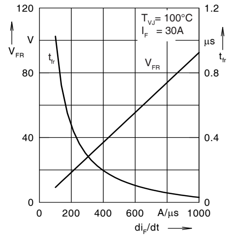
Fig. 18. Peak forward voltage V_{FR} and t_{fr} versus di_F/dt
