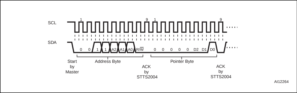
Figure 5. I 2 C write to pointer register
