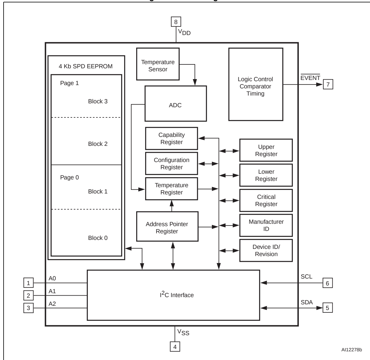
Figure 4. Block diagram
