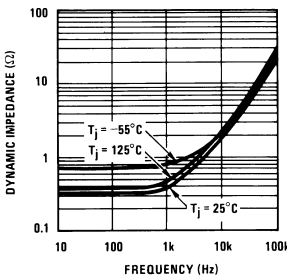
Dynamic Impedance
