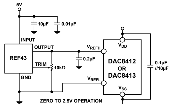
Figure 42. +5 V Single-Supply Operation
