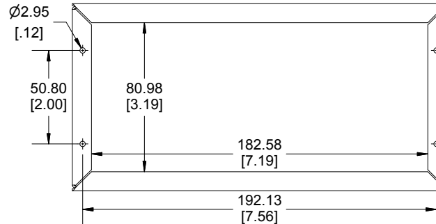
Bottom View of Chassis (Sold Separately)
