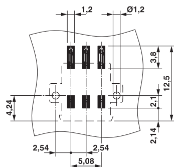
Drilling diagram
