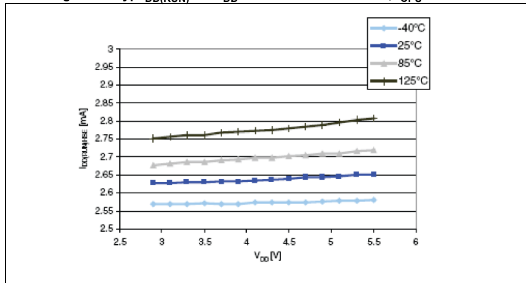
Figure 13. Typ I_{DD}(\text{RUN}) vs. V_{DD} HSE user external clock, f_{CPU} = 16 \text{ MHz}
