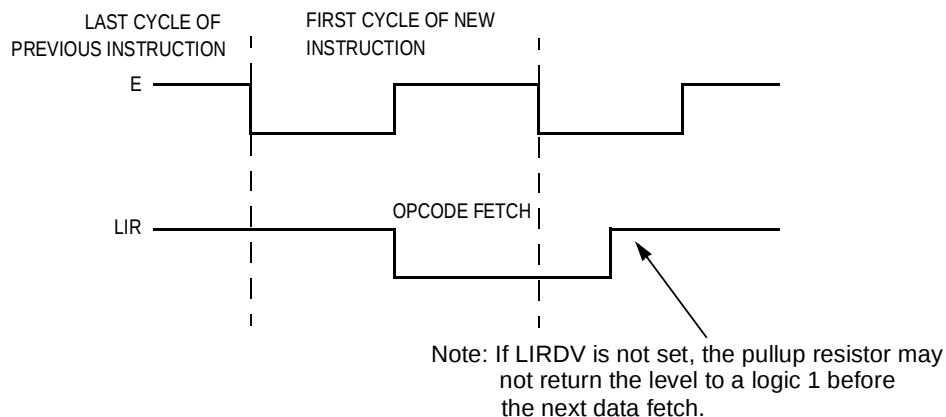
Figure 2-8. \overline{\text{LIR}} Timing
