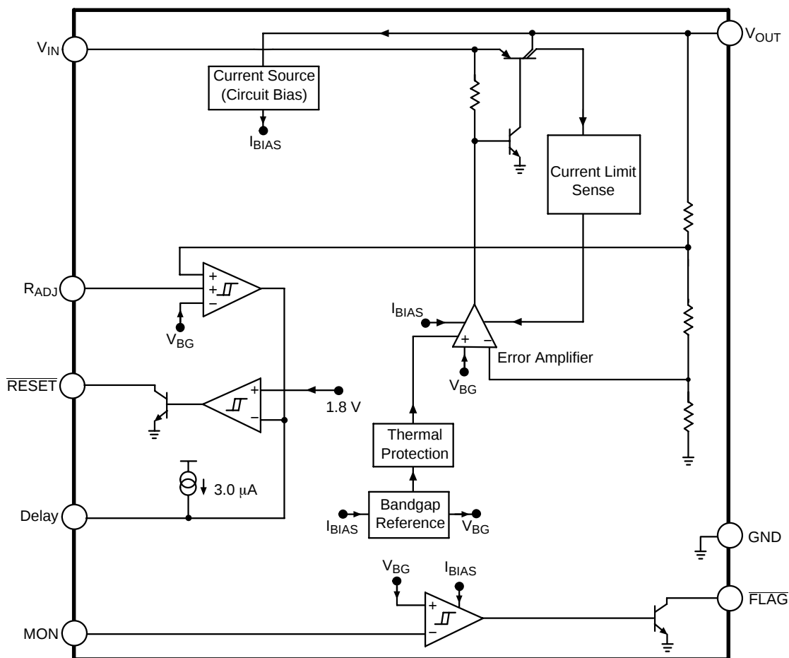
Figure 10. Block Diagram
