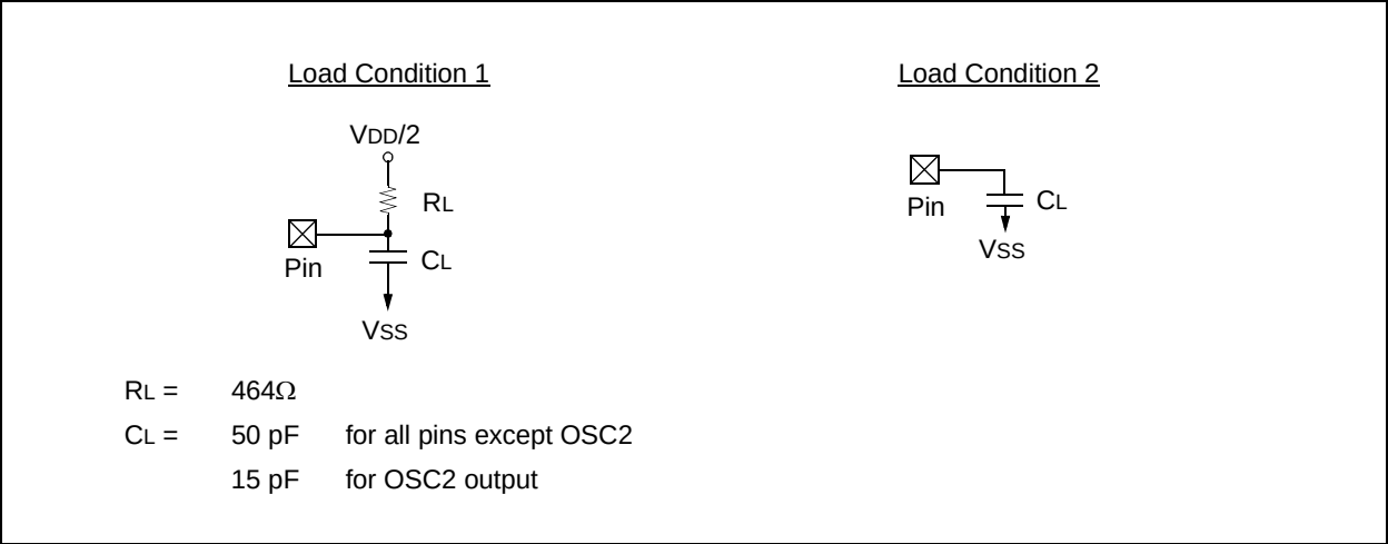
FIGURE 9-5: LOAD CONDITIONS
