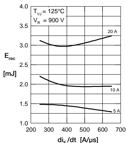
Fig. 6 Typ. recovery energy E_{rec} versus di_F/dt
