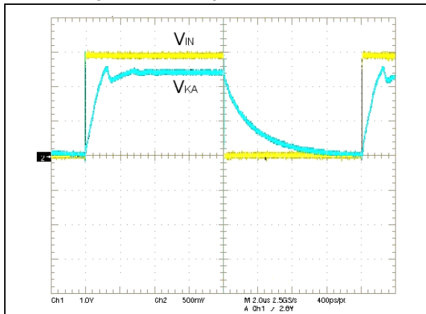
Figure 6. Startup characteristics
