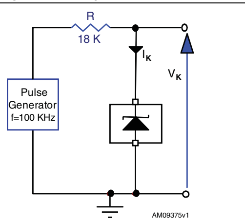
Figure 7. Startup measure circuit
