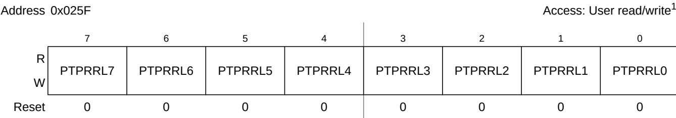
Figure 2-36. Port P Routing Register Low(PTPRRL)
