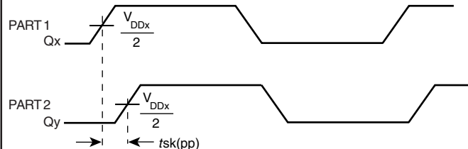
PART-TO-PART SKEW
