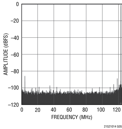
LTC2152-14: 32K Point FFT, f_{IN} = 122\text{MHz} , -1\text{dBFS} , 250Mps
