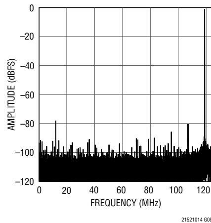
LTC2152-14: 32K Point FFT, f_{IN} = 381\text{MHz} , -1\text{dBFS} , 250Mps
