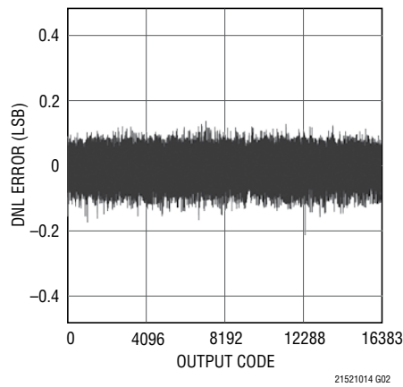
LTC2152-14: Differential Nonlinearity (DNL)
