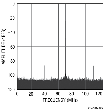
LTC2152-14: 32K Point FFT, f_{IN} = 70\text{MHz} , -1\text{dBFS} , 250Mps
