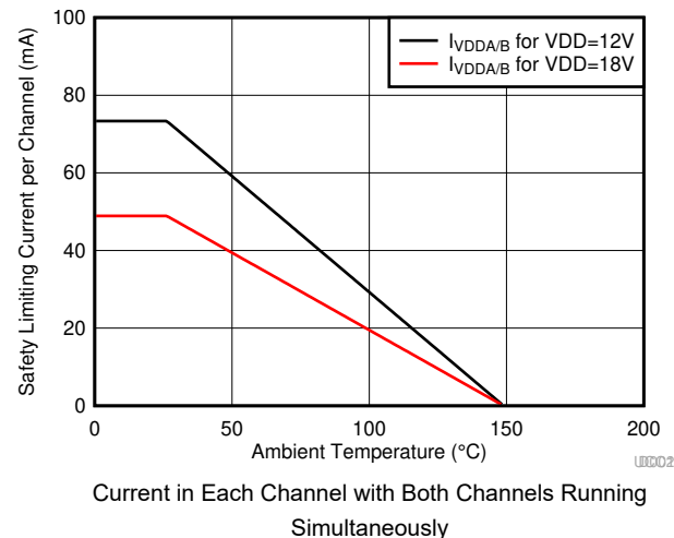
Figure 6-4. Thermal Derating Curve for Limiting Current Per VDE , DW Package
