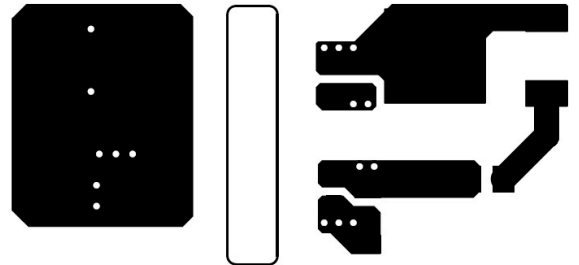
Figure 11-3. Bottom Layer Traces and Copper (Flipped)
