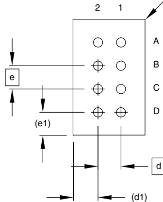
BOTTOM VIEW
