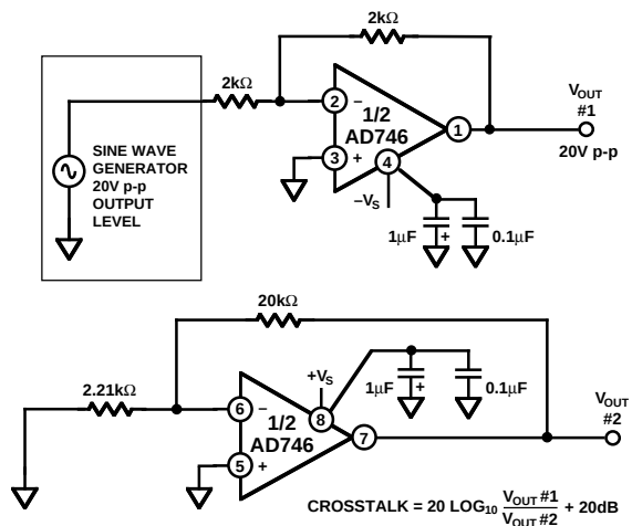
Figure 29. Crosstalk Test Circuit
