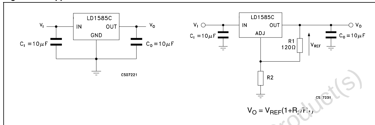
Figure 3. Application circuits
