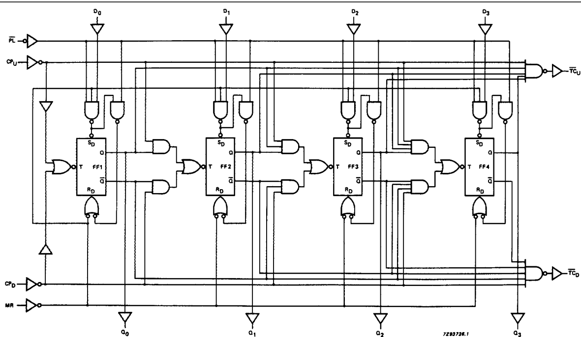
Fig.6 Logic diagram.
