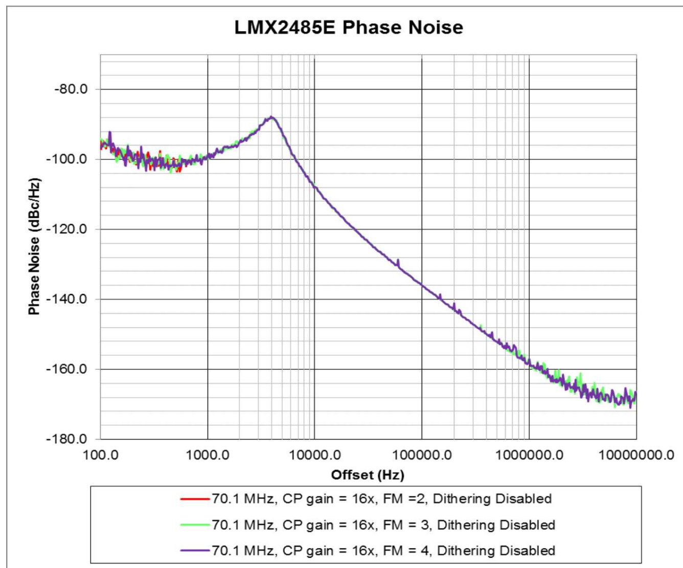
Figure 9. LMX2485E Impact of Fractional Modulator Order
