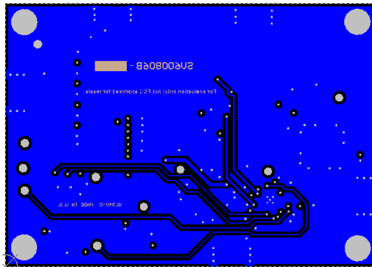
Figure 7. Layer #3 – Bottom Layer
