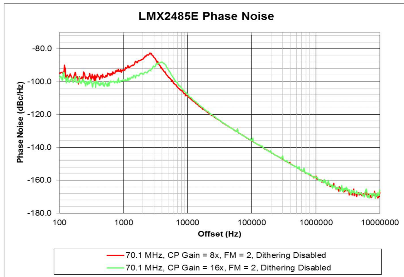
Figure 8. Impact of CPG on Phase Noise
