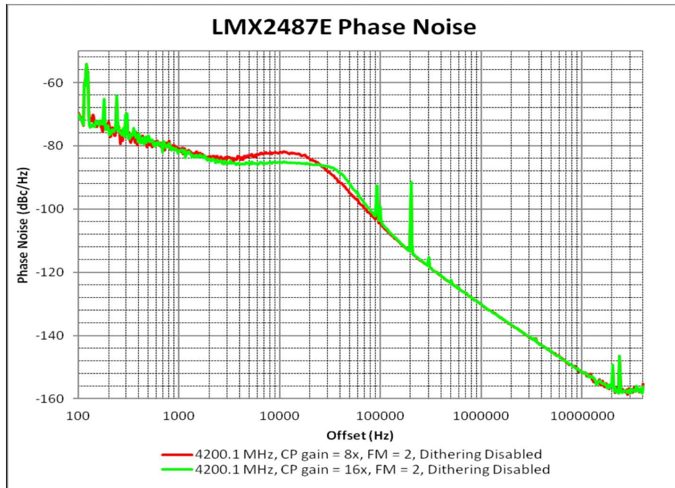
Figure 11. LMX2487E Impact of CPG on Phase Noise
