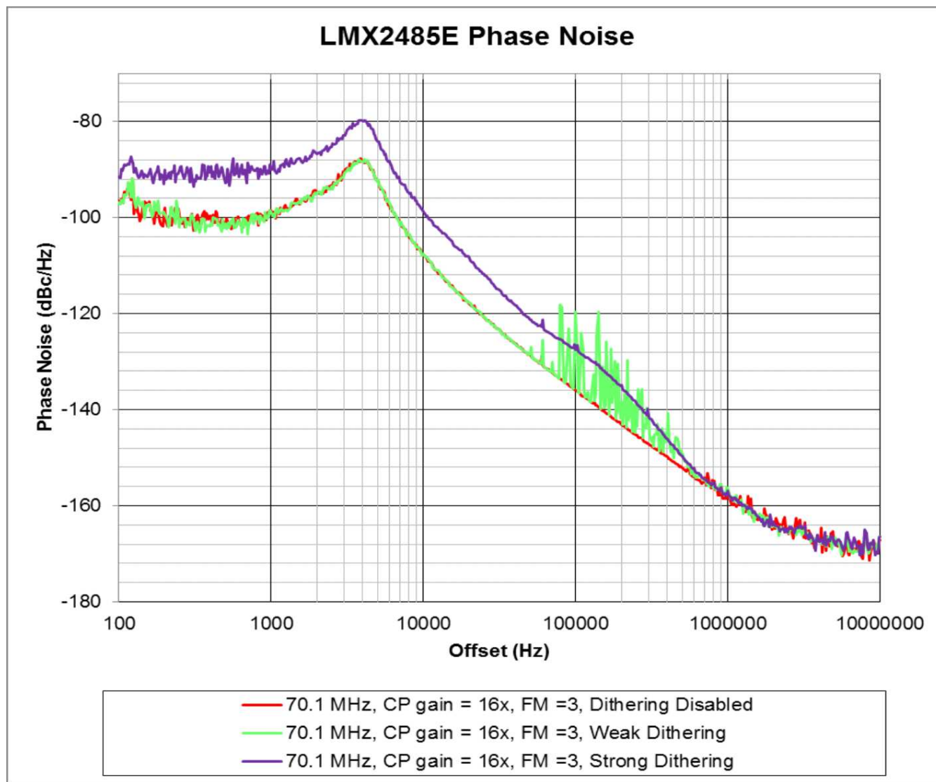
Figure 10. LMX2485E Impact of Dithering
