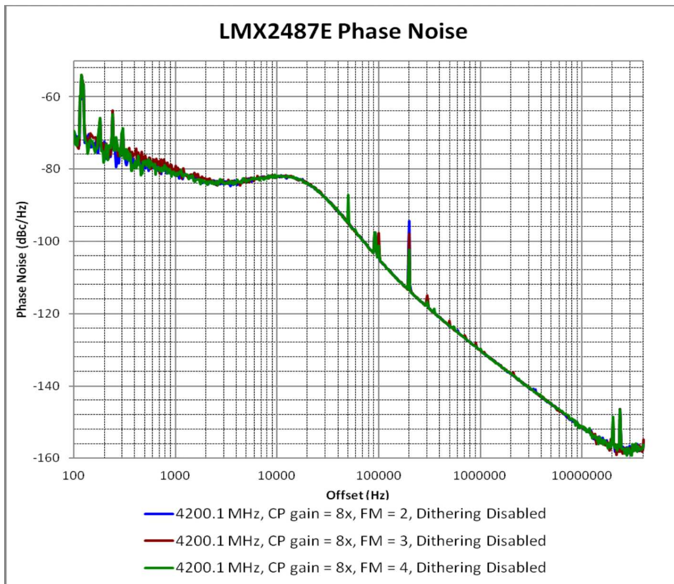
Figure 12. LMX2487E Impact on Fractional Modulator
