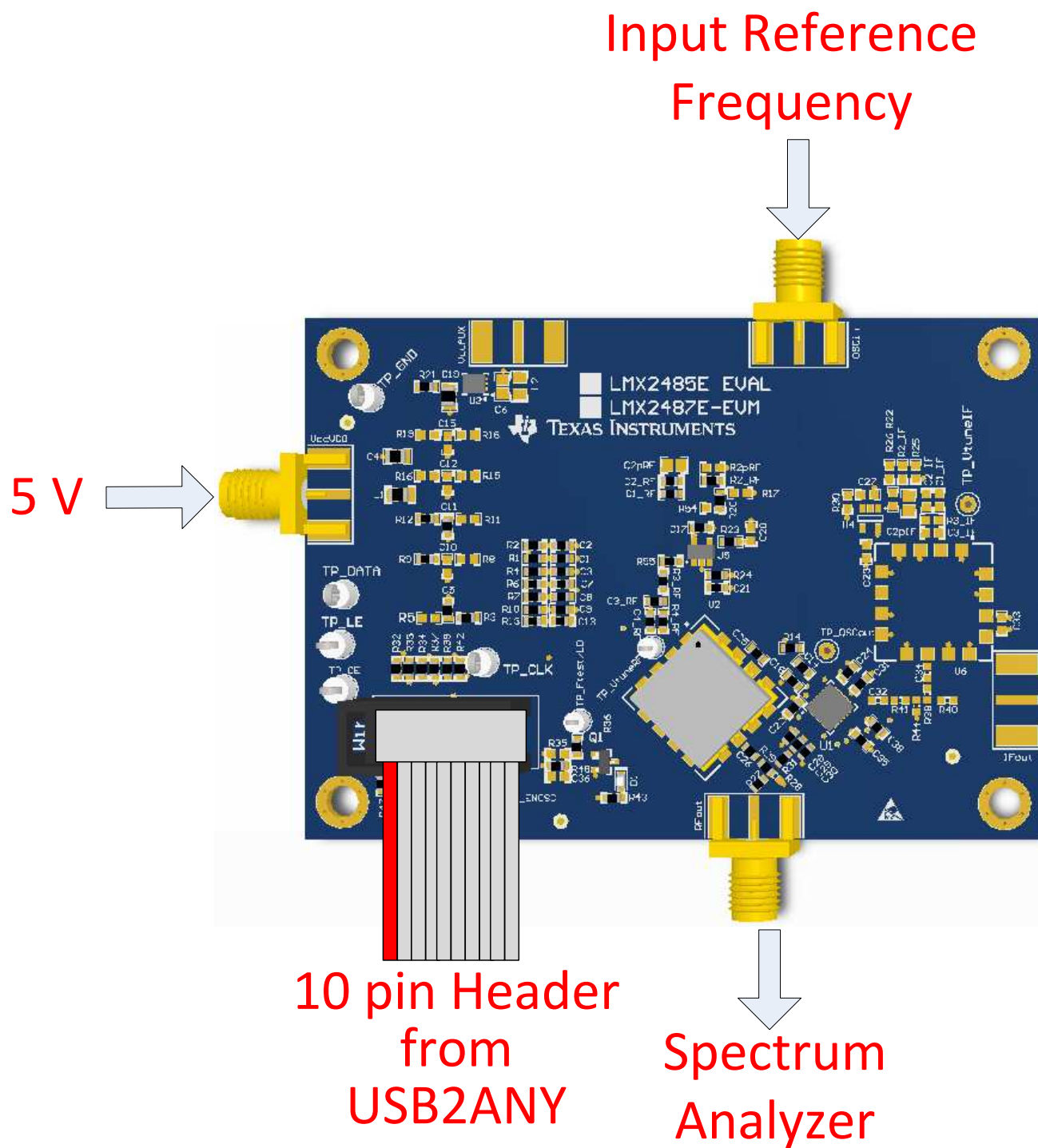
Figure 1. Evaluation Board Setup
