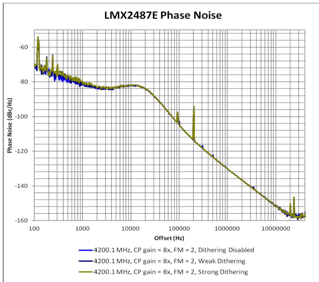
Figure 13. LMX2487E Impact of Dithering
