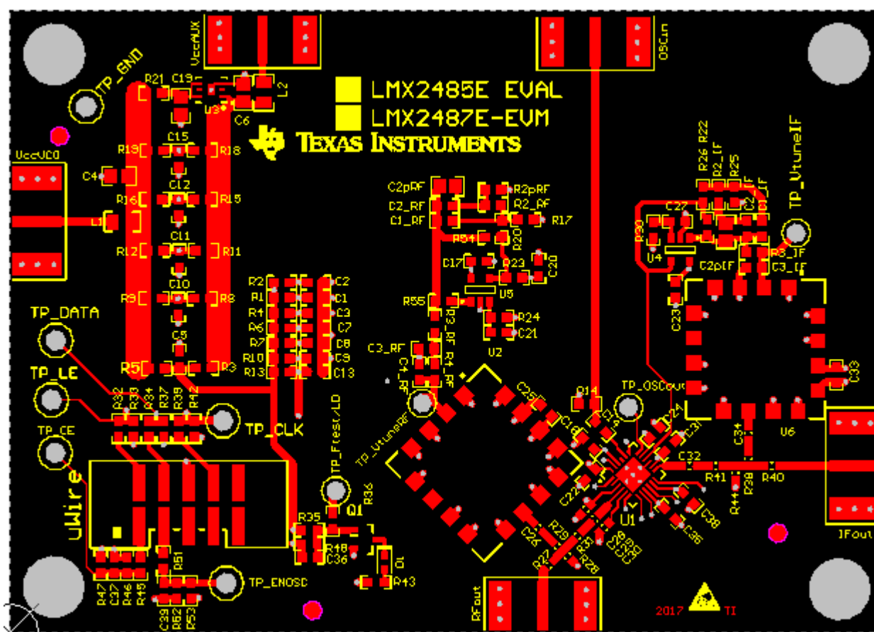
Figure 4. Layer #1 – Top
