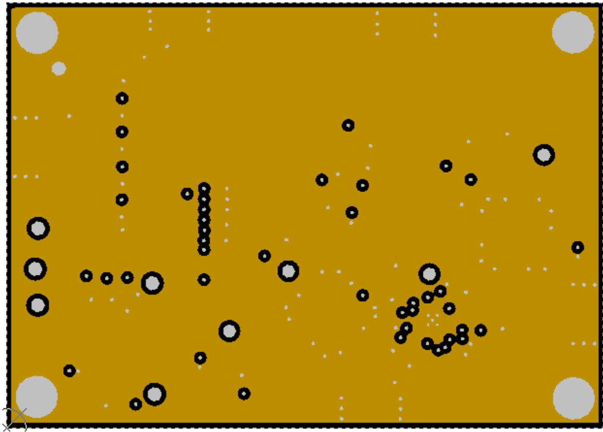
Figure 5. Layer #2 – RF Ground Plane
