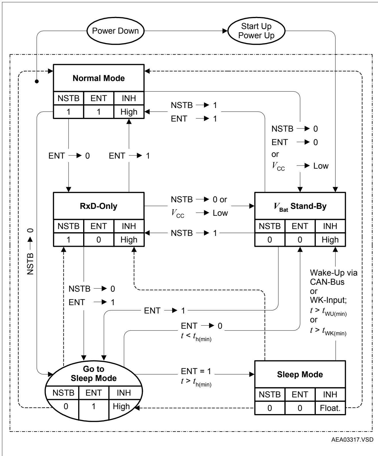
Figure 3 State Diagram
