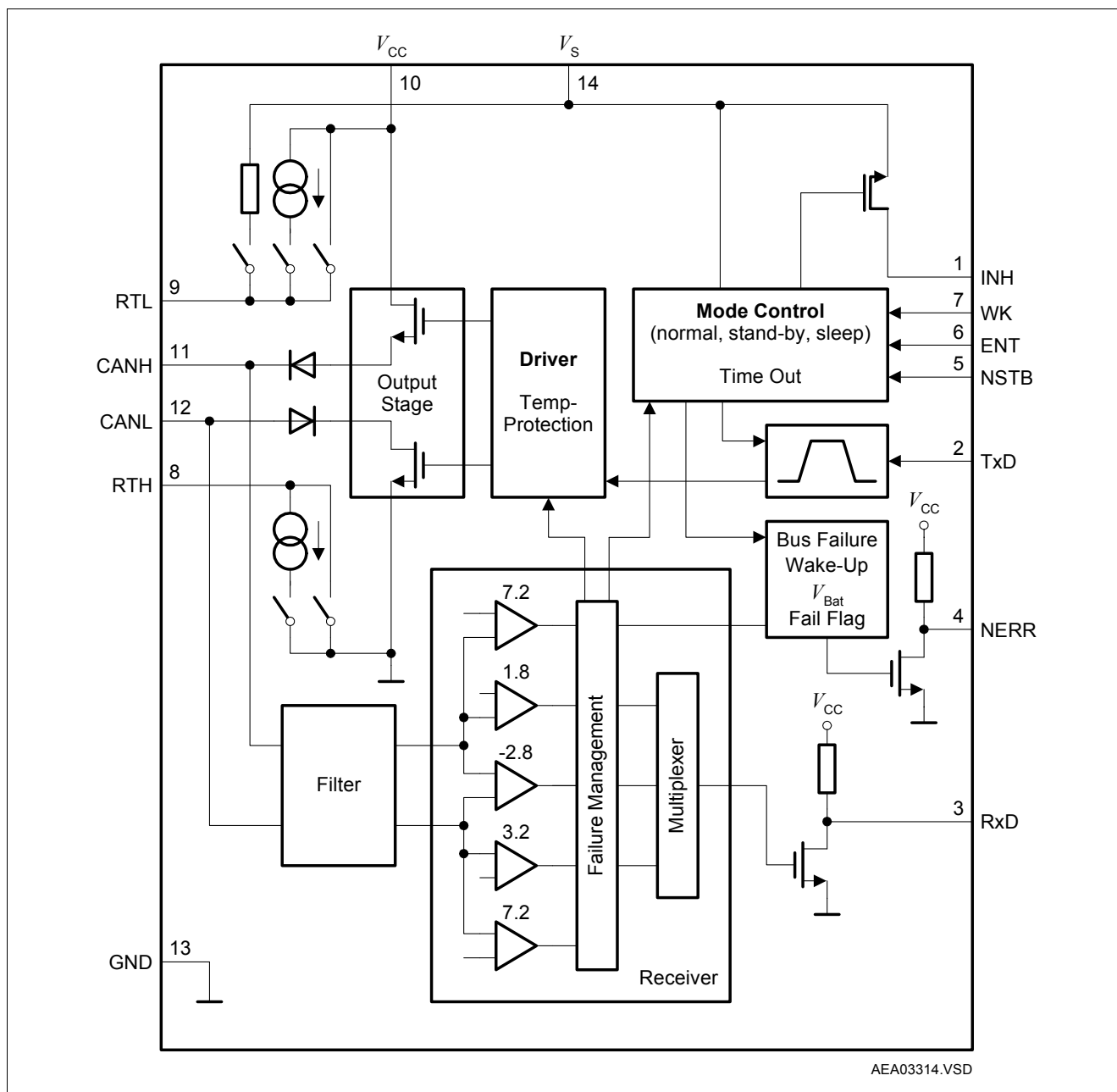
Figure 1 Block Diagram
