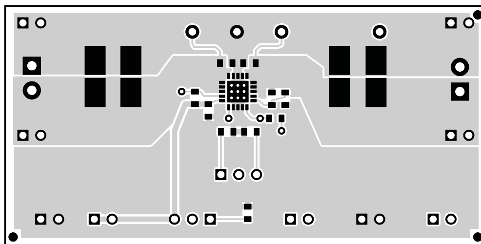
Figure 6. Top Layer
