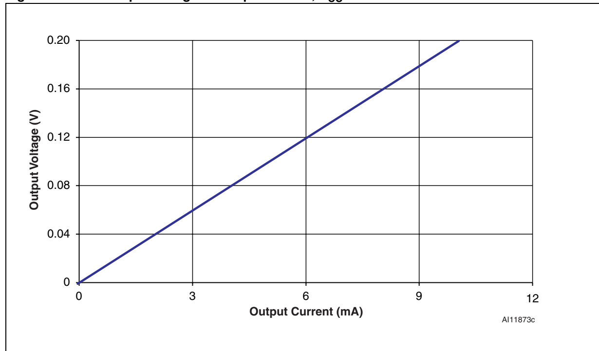
Figure 9. \overline{\text{RST}} output voltage vs. output current, V_{CC} = 4.25\text{V}
