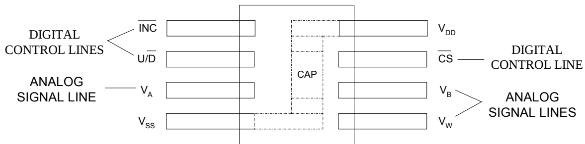
FIGURE 9 – WMS7120/1 LAYOUT
