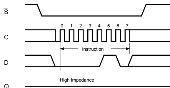
Figure 6. Write enable (WREN) sequence
