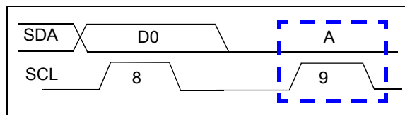
FIGURE 6-4: Acknowledge Waveform.
